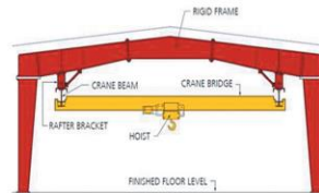
UNDERHUNG CRANE
