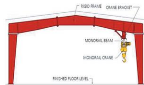
MONORAIL CRANE
